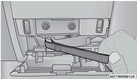
Manual Park Release Tether
